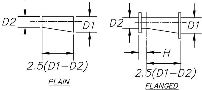
PLAIN FLANGED ECCENTRIC REDUCER
