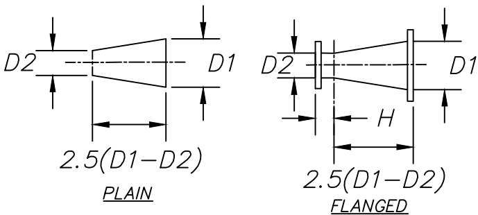
PLAIN FLANGED CONCENTRIC REDUCER
