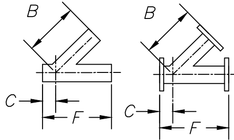
PLAIN FLANGED 45° LATERAL
