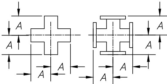
PLAIN FLANGED CROSS
