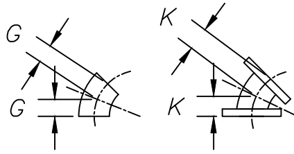
PLAIN FLANGED 45° ELBOW
